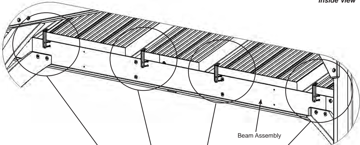
Fig. 22.1 Inside View
